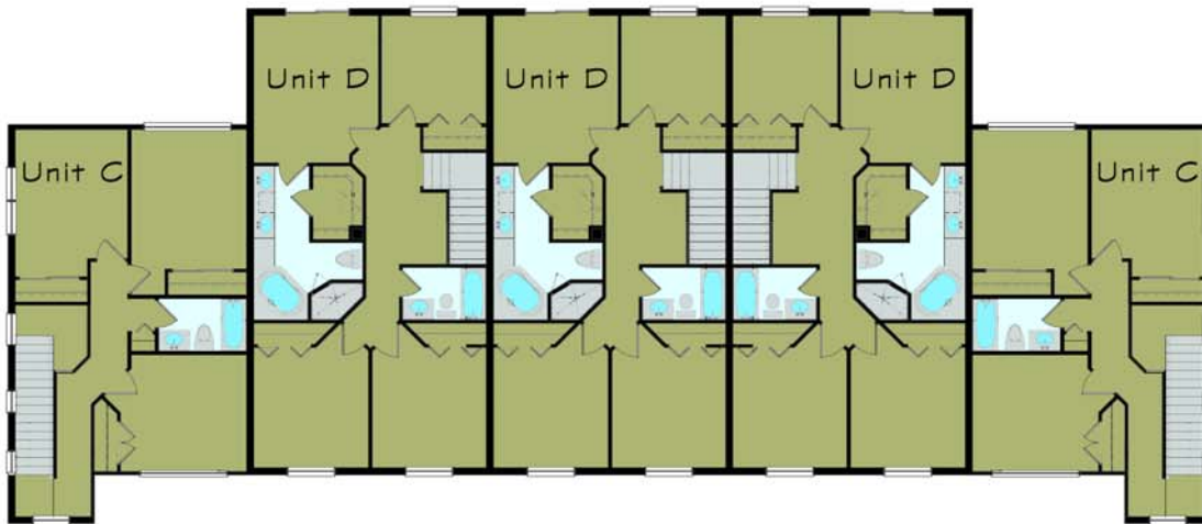
SECOND FLOOR OF FIVE UNIT BUILDING
